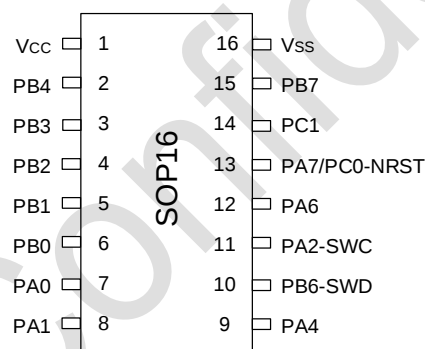
图 3-2 SOP16 Pinout1 PY32F002BW15S7-C (Top view)
